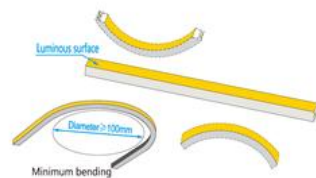
Bending Diagram
