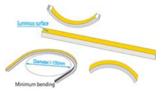
Bending Diagram
