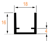
Aluminium Profile
