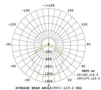
Photometry L1200
